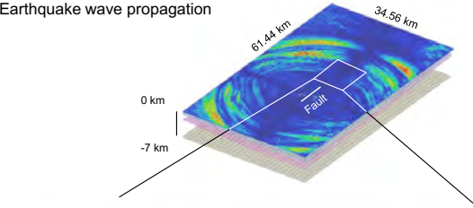
a) Earthquake wave propagation
